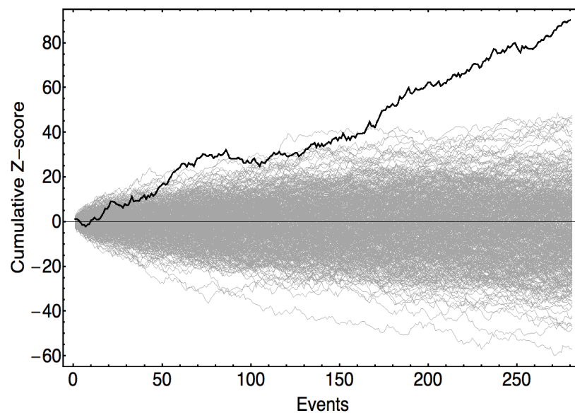
Figure 4: The bold line shows the cumulative deviation of results for formal trials, compared with 500 resampling datasets using the same event sequence, but with randomly offset start times.
