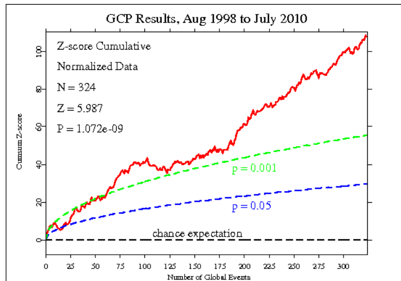
Figure 5: Cumulative deviation of 324 formal events, spanning August 1998 to July 2010. The data show consistent deviation, and the terminal value of the accumulation is approximately 6 standard deviations, corresponding to chance odds of 1 in 10^9 .
