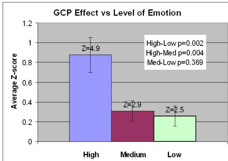
Figure 6. Level of emotion determined by categorizing the events significantly affects the network variance effect size.
