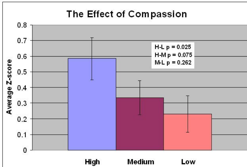
Figure 7. The degree of compassion evoked or embodied in an event significantly affects the network variance effect size.
